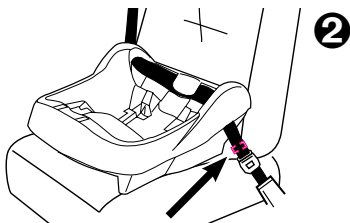
Locking clip goes here, 1/2 inch from the buckle
